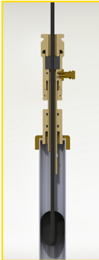
Cross section of ECV Exchange Kit showing inflated balloon.
