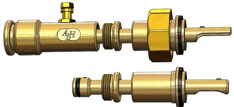
The interchangeable attachments of the ECV Exchange Kit.
